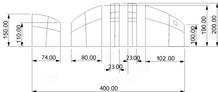
Obr. 42: Bokorys
